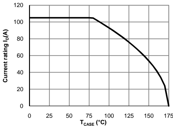
Figure 14: Current De-rating (Note E)
