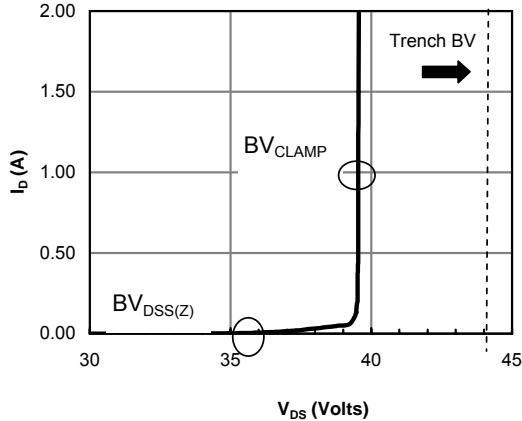
Fig 15: BV CLAMP Characteristic
