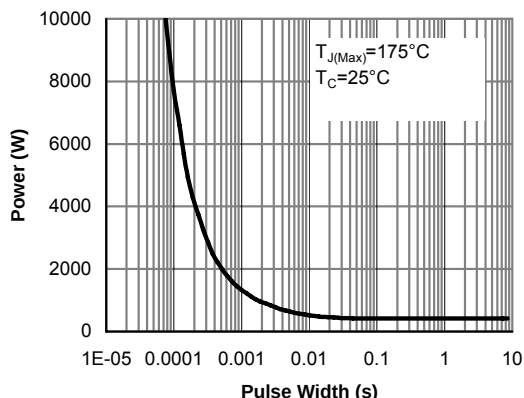
Figure 10: Single Pulse Power Rating Junction-to-Case for AOT474 (Note F)
