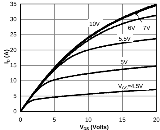
Figure 2: On-Region Characteristics@125°C
