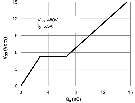
Figure 8: Gate-Charge Characteristics
