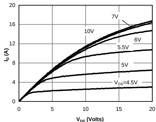
Figure 2: On-Region Characteristics@125°C
