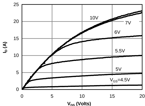
Figure 1: On-Region Characteristics@25°C
