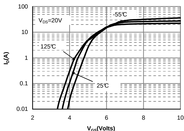
Figure 3: Transfer Characteristics
