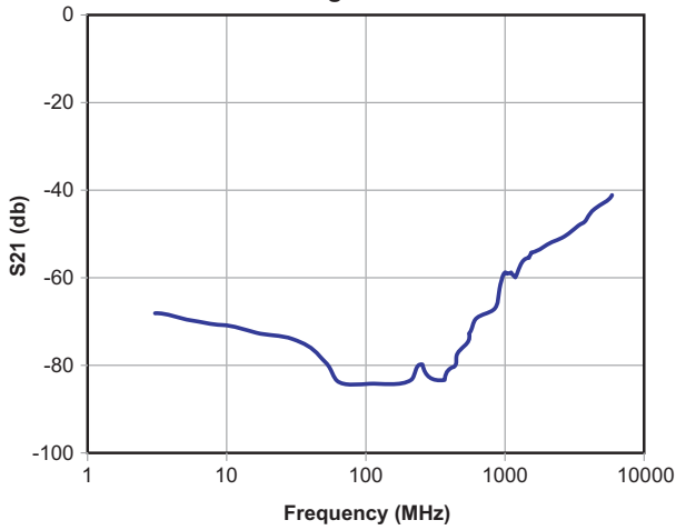
Analog Crosstalk
