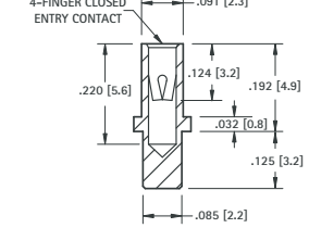
.032 (.81) - .046 (1.17) PIN - SOLDER MOUNT
