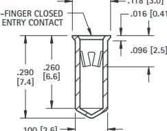
.040 (1.02) - .050 (1.27) PIN - SOLDER MOUNT
