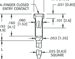
IC SOCKET CONTACTS FOR .015 (.38) - .025 (.64) LEADS - PRESS-FIT
