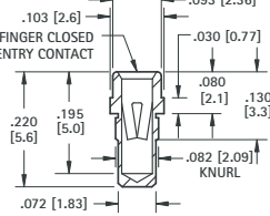
.032 (.81) - .046 (1.17) PIN - PRESS-FIT
