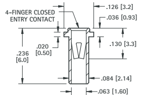
.032 (.81) - .046 (1.17) PIN - SOLDER MOUNT
