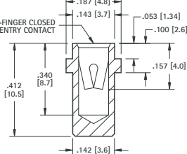
.065 (1.65) - .082 (2.08) PIN - SOLDER MOUNT
