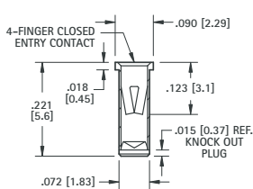
.032 (.81) - .046 (1.17) PIN - SOLDER MOUNT
