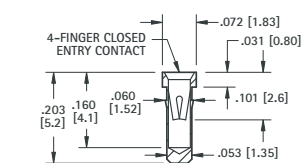
IC SOCKET CONTACTS FOR .015 (.38) - .025 (.64) LEADS - PRESS-FIT
