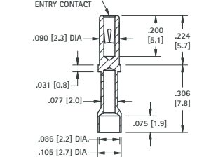
.032 (.81) - .046 (1.17) PIN - CRIMP BARREL JACK
