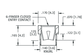
.084 (2.13) - .102 (2.6) PIN - PRESS-FIT
