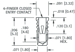
.032 (.81) - .046 (1.17) PIN - PRESS-FIT
