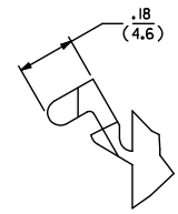
DETAIL B PREBENT MOUNTING EAR (SCALE 4:1)
