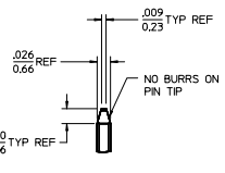
DETAIL X SCALE 5:1 SEE NOTE 10
