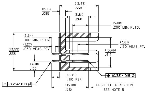
SECTION W-W
