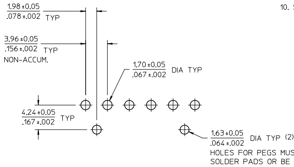
PCB LAYOUT: COMPONENT SIDE
