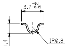
SECT. C-C
