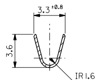
SECT. A-A
