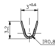
SECT. B-B
