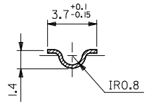
SECT. C-C
