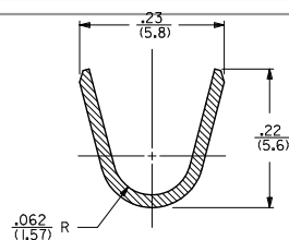
SECTION C-C SCALE 8:1
