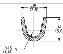
SECTION B-B SCALE 8:1 18-16 AWG WIRE
