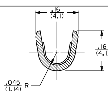
SECTION B-B SCALE 8:1 14 AWG WIRE
