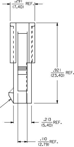
5559-03P3-225 WITHOUT MOUNTING EARS
