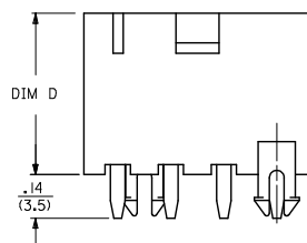
CIRCUIT NO. 1 .1654±.015 (4.200±0.38) TYP.
