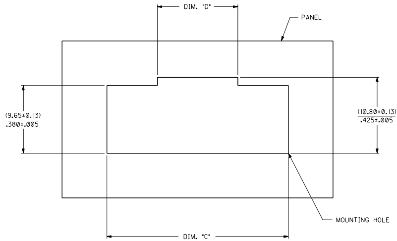
OPTION "A" RECOMMENDED MOUNTING HOLE LAYOUT
