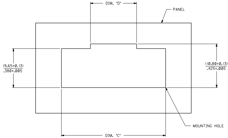
OPTION "A" RECOMMENDED MOUNTING HOLE LAYOUT
