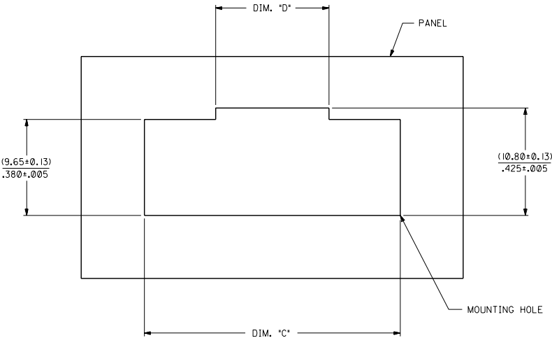
OPTION "A" RECOMMENDED MOUNTING HOLE LAYOUT
