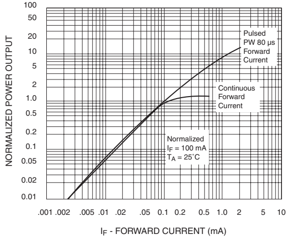
Fig. 1 Power Output vs. Input Current
