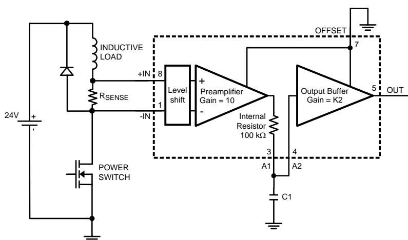
Figure 62. Low-Side Current-Sensing Application
