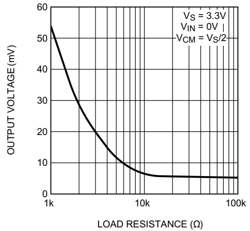
Figure 32. Negative Swing vs R_{\text{LOAD}} at V_S = 3.3\text{ V}
