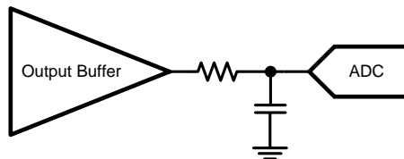
Figure 59. Reduce Error When Driving ADCs
