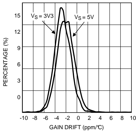
Figure 39. Gain Drift Distribution, 5000 Parts LMP8602 and LMP8602-Q1
