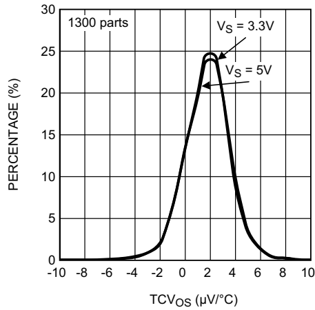
Figure 37. TCV 0S Distribution
