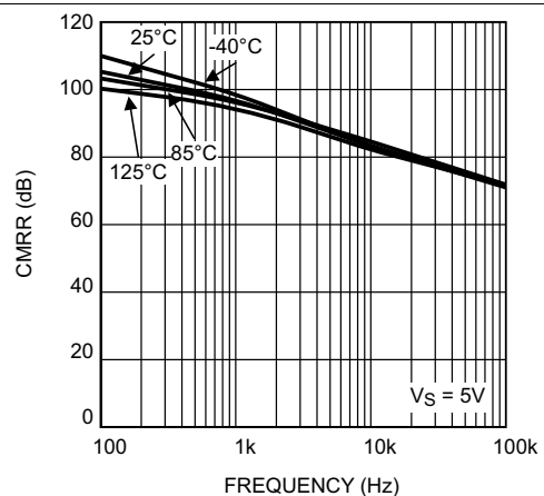
Figure 12. CMRR vs Frequency at V_S = 5\text{ V}
