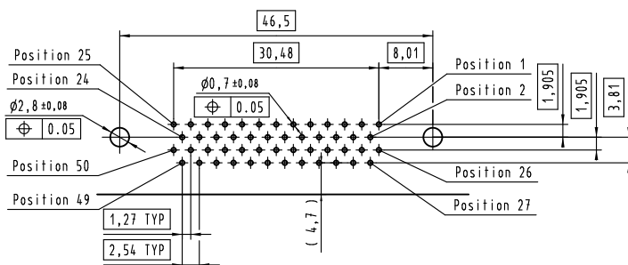
PCB layout: component side
