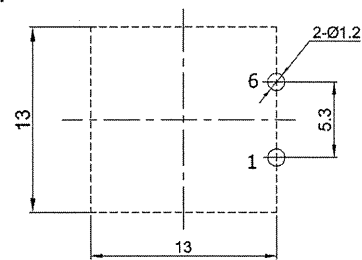
P.C.B.LAYOUT(BottomView)
