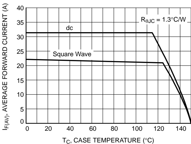
Figure 5. Current Derating
