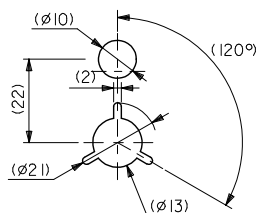
DETAIL "H"
