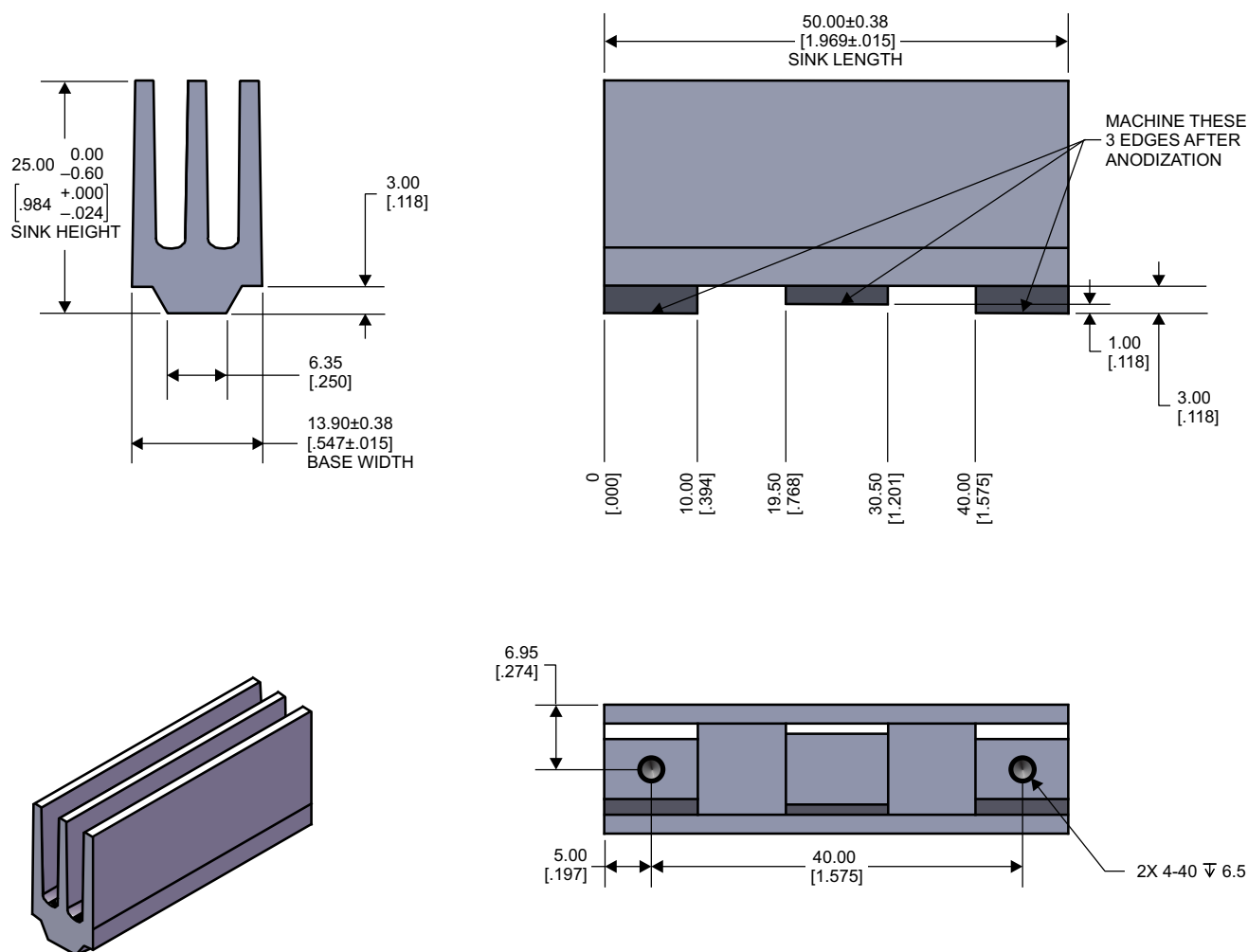
Figure 42. EVM Heatsink
