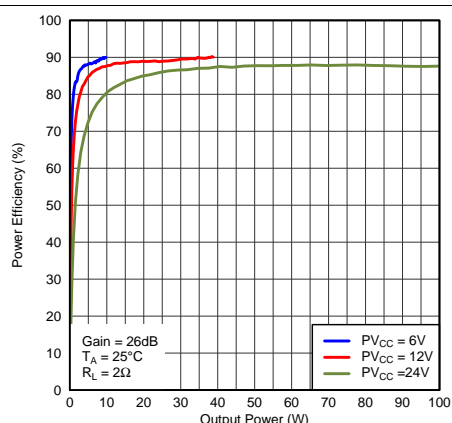
Figure 23. Power Efficiency (PBTL) vs Output Power
