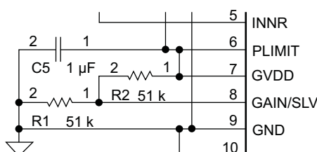
Figure 27. Gain, Master/Slave
