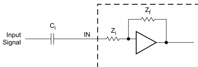
Figure 28. Input Impedance
