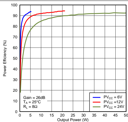
Figure 15. Power Efficiency (BTL) vs Output Power
