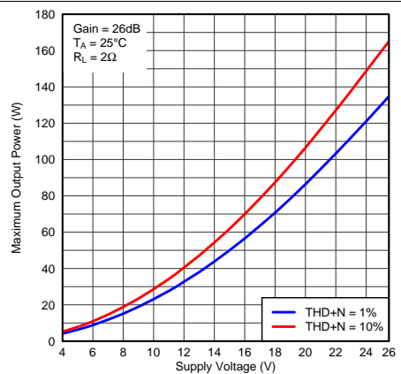
Figure 22. Maximum Output Power (PBTL) vs Supply Voltage
