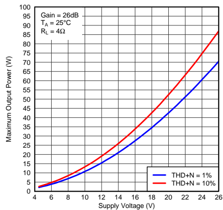
Figure 14. Maximum Output Power (BTL) vs Supply Voltage
