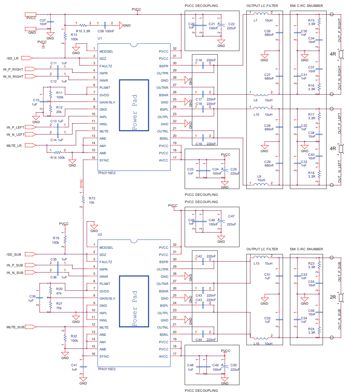
Figure 37. Schematic
