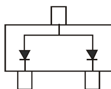
BAT54AW-KL6
