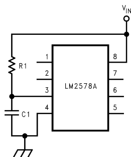
Figure 22. Maximum Duty Cycle Limiting
