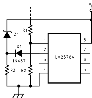
Figure 21. Under-Voltage Lockout
