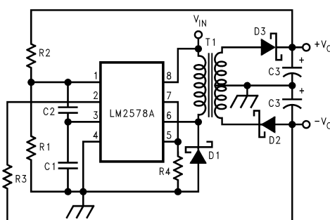
Figure 35. Buck-Boost Regulator
