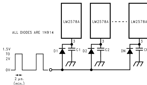
Figure 26. Synchronizing Devices
