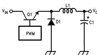
Figure 27. Basic Buck Regulator
