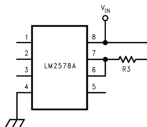
Figure 16. Current Limit, V_{in} Referred
