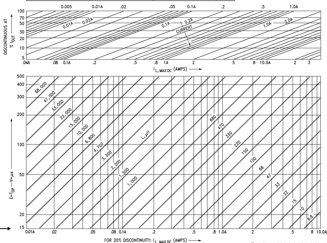
Figure 29. DC/DC Inductance Calculator
