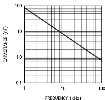
Figure 14. Value of Timing Capacitor vs Oscillator Frequency
