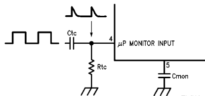
FIGURE 2. Monitoring Square Wave μP Signals
