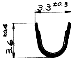
SECT. "B" - "B"
