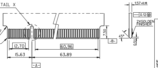
RECOMMENDED MATING P.C.BOARD EDGE CONFIGURATION
