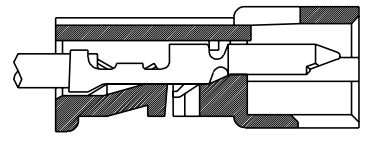
断面E-E SECT. E-E
