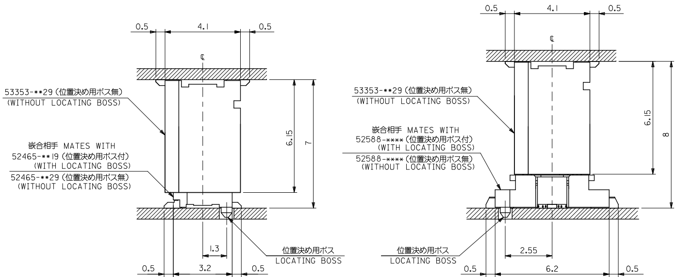
嵌合状態図 (参考) MATED DRAWING (REF.)
