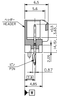
SECT H-H
