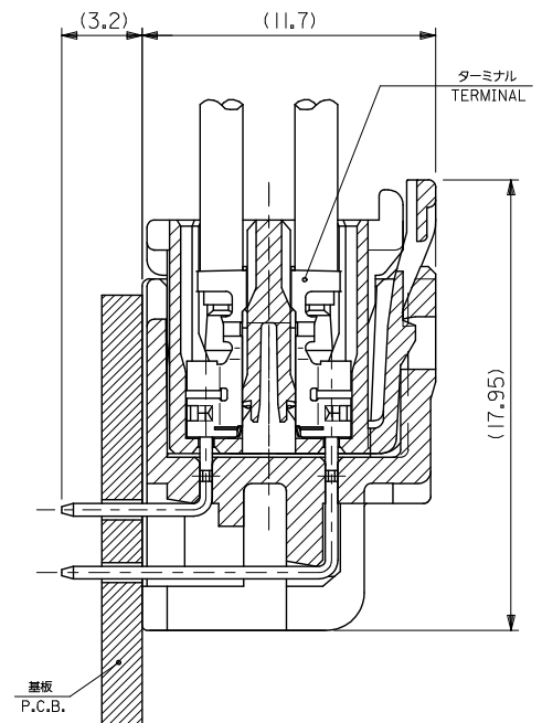
嵌合断面図 (参考) MATED DRAWING (REF.)
