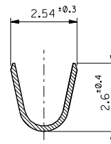
SECT. Y-Y
