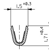
SECT. Z-Z
