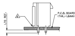
RECOMMENDED INSTALLATION PATTERN
