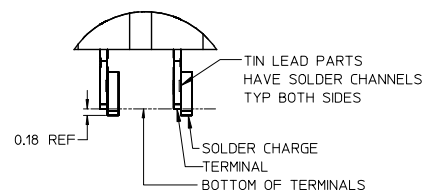
SOLDER CHARGE DETAIL
