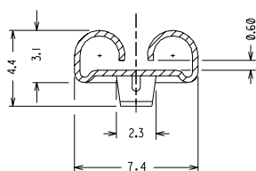
SECTION A - A
