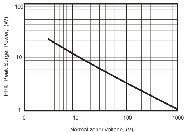
Fig.2- Maximum Non-repetitive Surge Power
