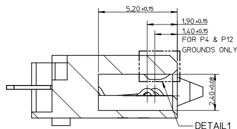
SECTION Z-Z
