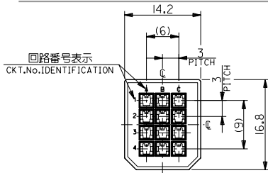
嵌合側 MATING SIDE
