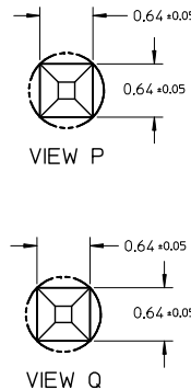
RECOMMENDED PCB HOLE LAYOUT
