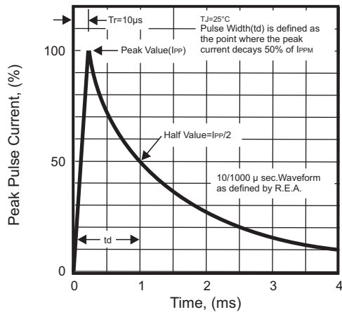
Fig. 3 - Pulse Waveform
