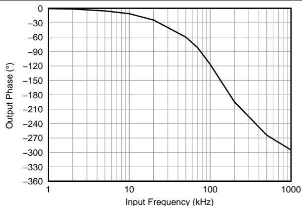
Figure 13. Output Phase vs Input Frequency
