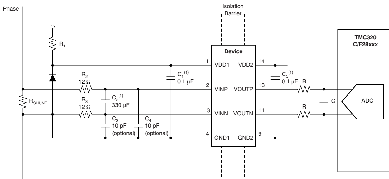
Figure 34. Shunt-Based Current Sensing with the AMC1100
