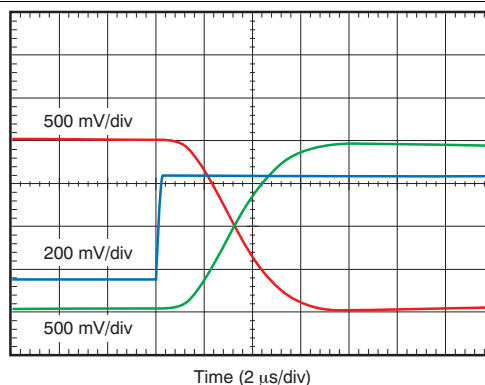
Figure 35. Typical Step Response of the AMC1100
