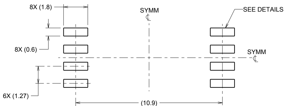
LAND PATTERN EXAMPLE 9.1 mm NOMINAL CLEARANCE/CREEPAGE SCALE:6X
