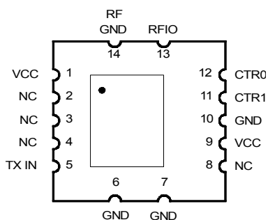
DR4001 Pin Out
