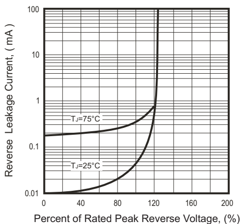
Fig.5- Reverse Characteristics
