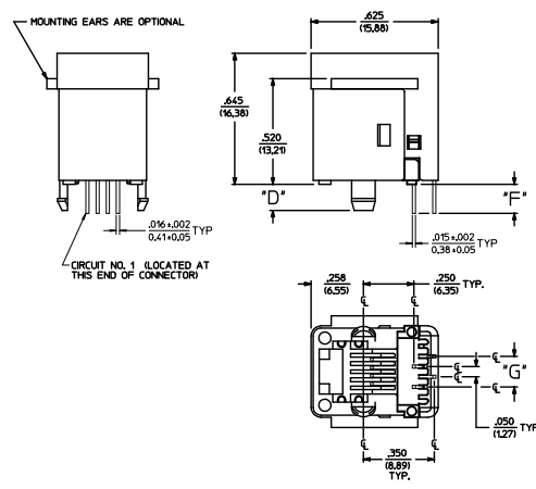
SIZE 4 MODULAR JACK LOADED WITH 4 TERMINALS SHOWN ABOVE (SEE SHEET 4 FOR PART NUMBER AVAILABILITY)
