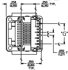
SIZE 8 MODULAR JACK LOADED WITH 8 TERMINALS SHOWN ABOVE (SEE SHEET 4 FOR PART NUMBER AVAILABILITY)
