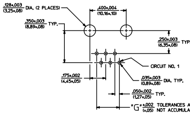
P.C. BOARD LAYOUT FOR CONNECTOR SIZE 6
